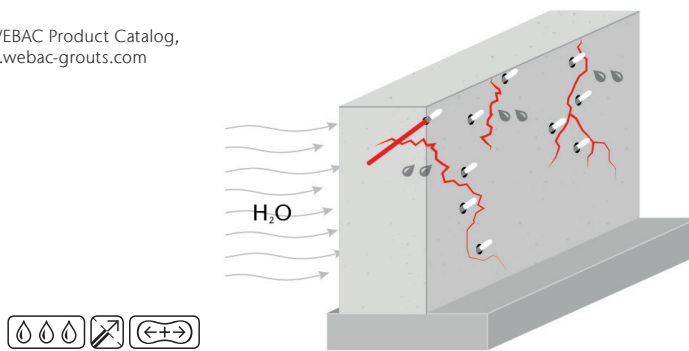
Crack repair in concrete under hydrostatic pressure
